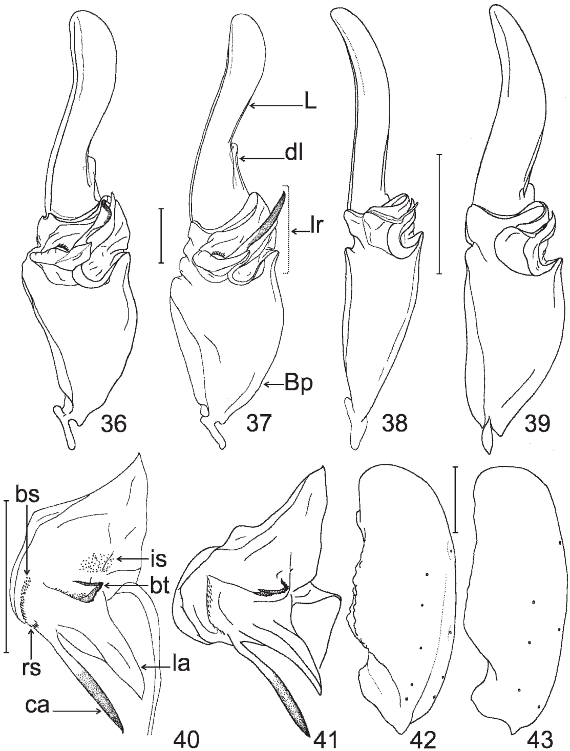
Figs. 36-43. Diagnostic characters of Chilean Brachistosternus Pocock, 1893. 36, 42. Brachistosternus ( B. ) ehrenbergii (Gervais, 1841). 36. Sinistral hemispermatophore, internal aspect. 42. Sinistral pedipalp
